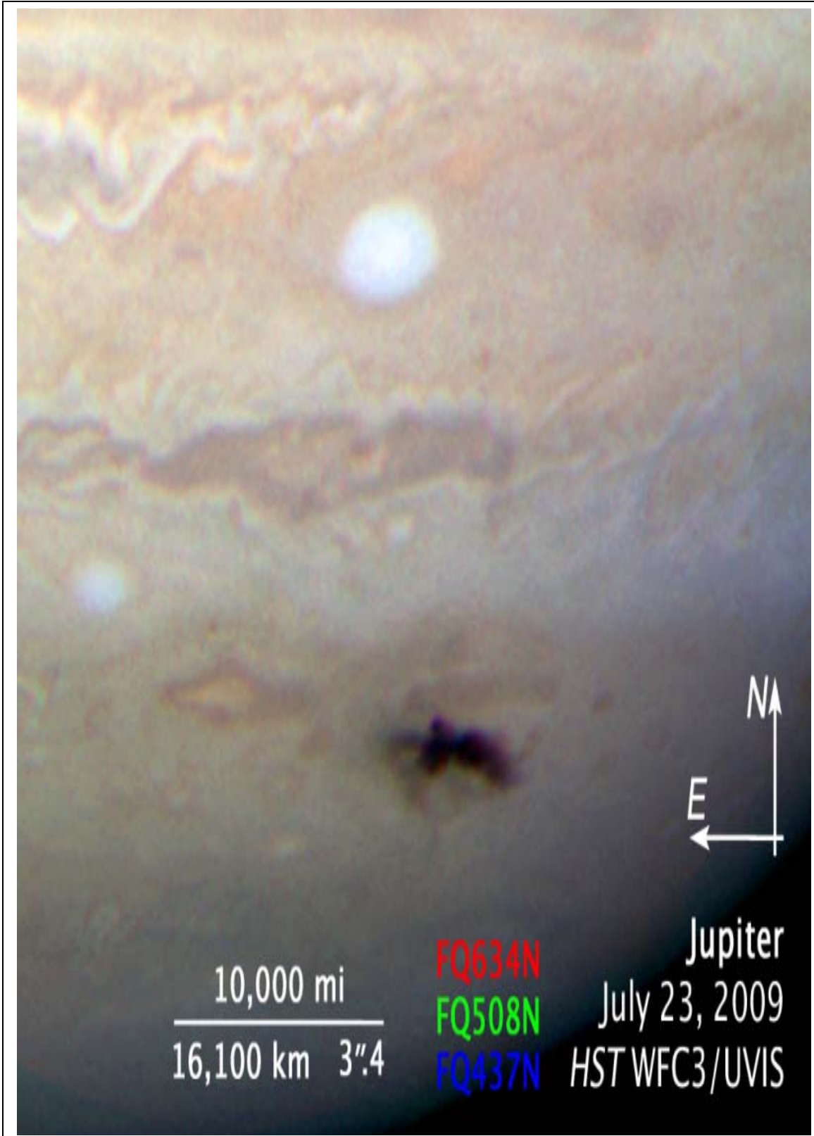
Photo copyright 2009 JPL/NASA from the Hubble Space Telescope. Exercise copyright 2009 The Classroom Astronomer in Issue #1.
